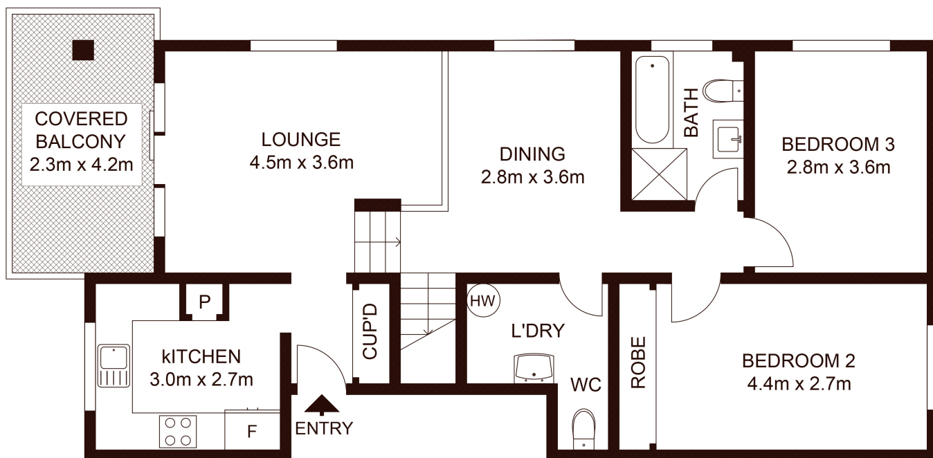
TOP FLOOR
