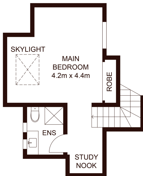
UPPER FLOOR
